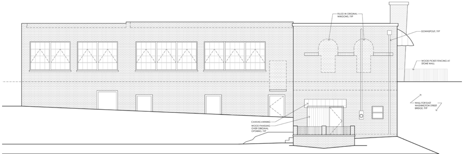
2 EXISTING LEFT SIDE ELEVATION 1/4" = 1'-0"
